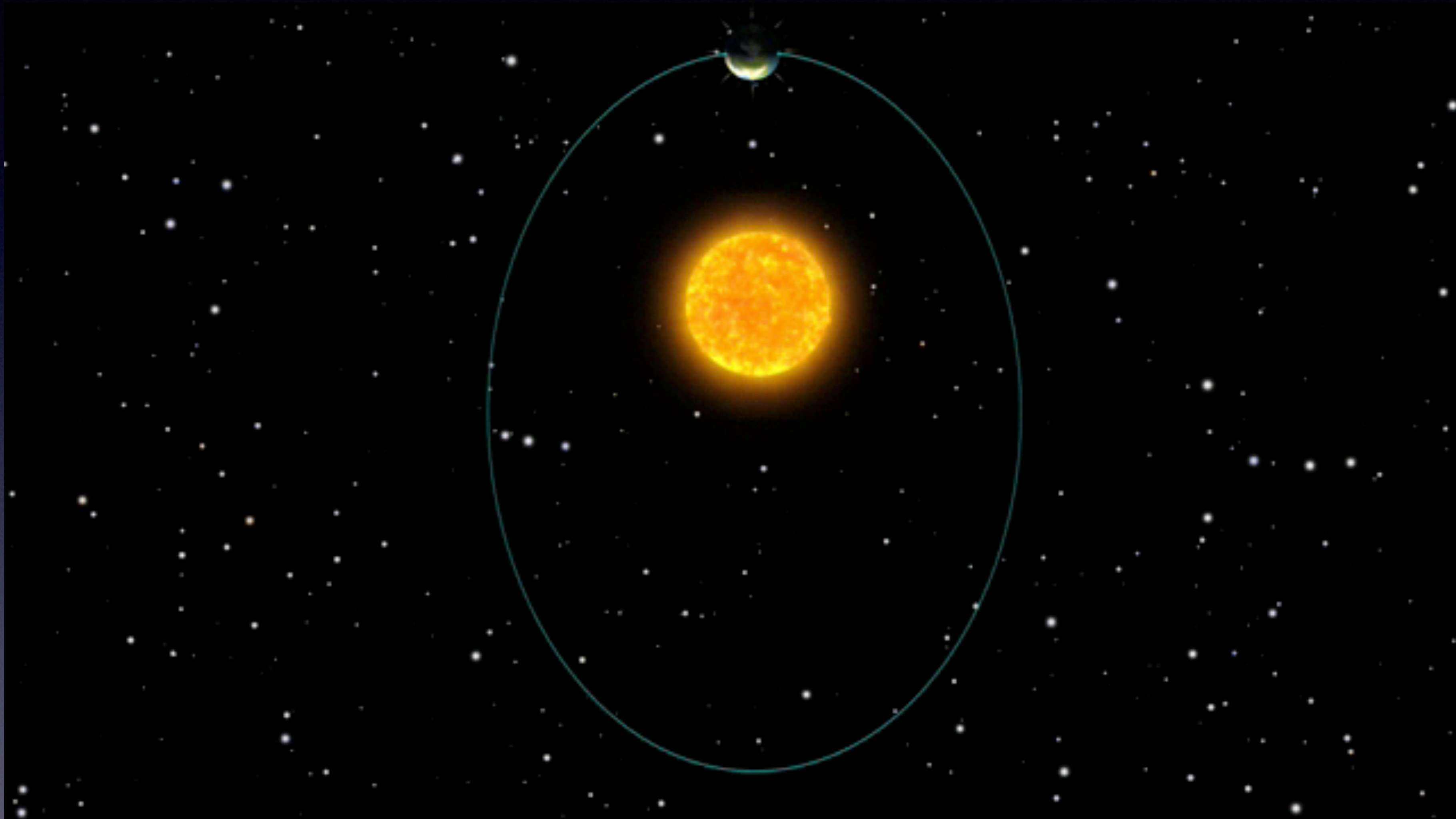
Earth's Revolution
